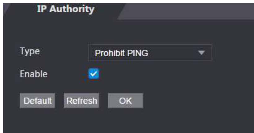
Figure 3-41 Prohibit PING
