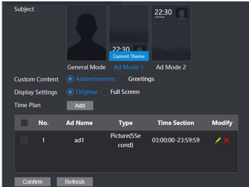
Figure 3-20 Ad mode
