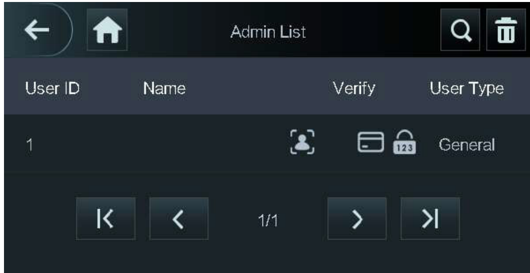
Figure 2-9 Admin list
