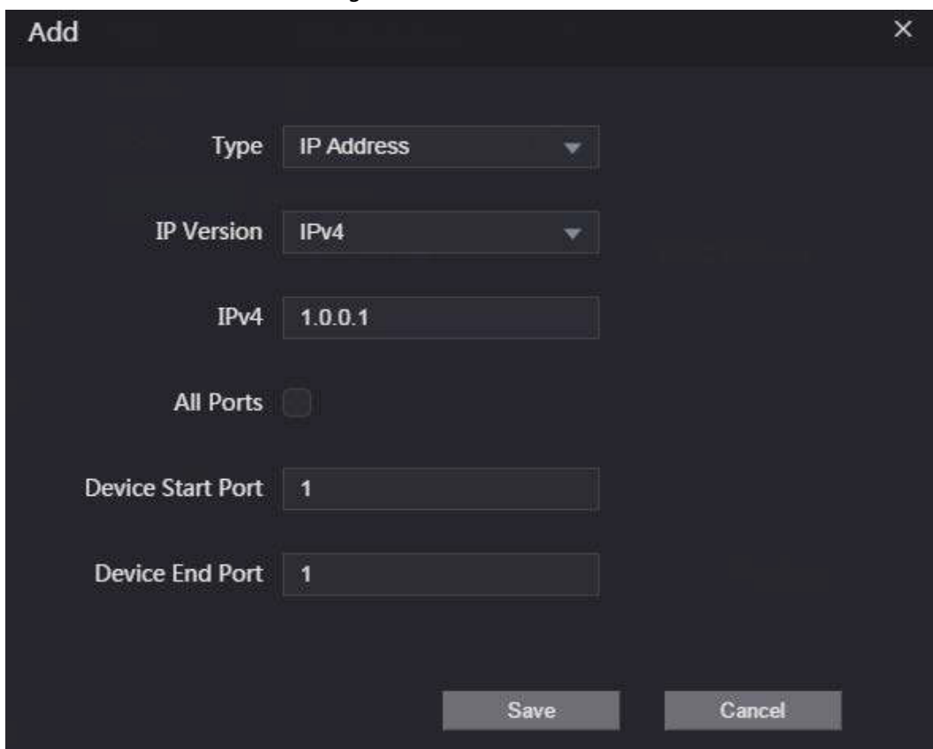
Figure 3-40 Add IP
