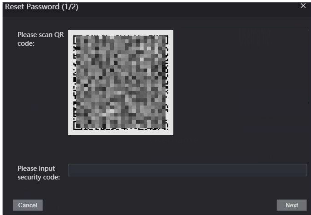
Figure 3-2 Reset password
