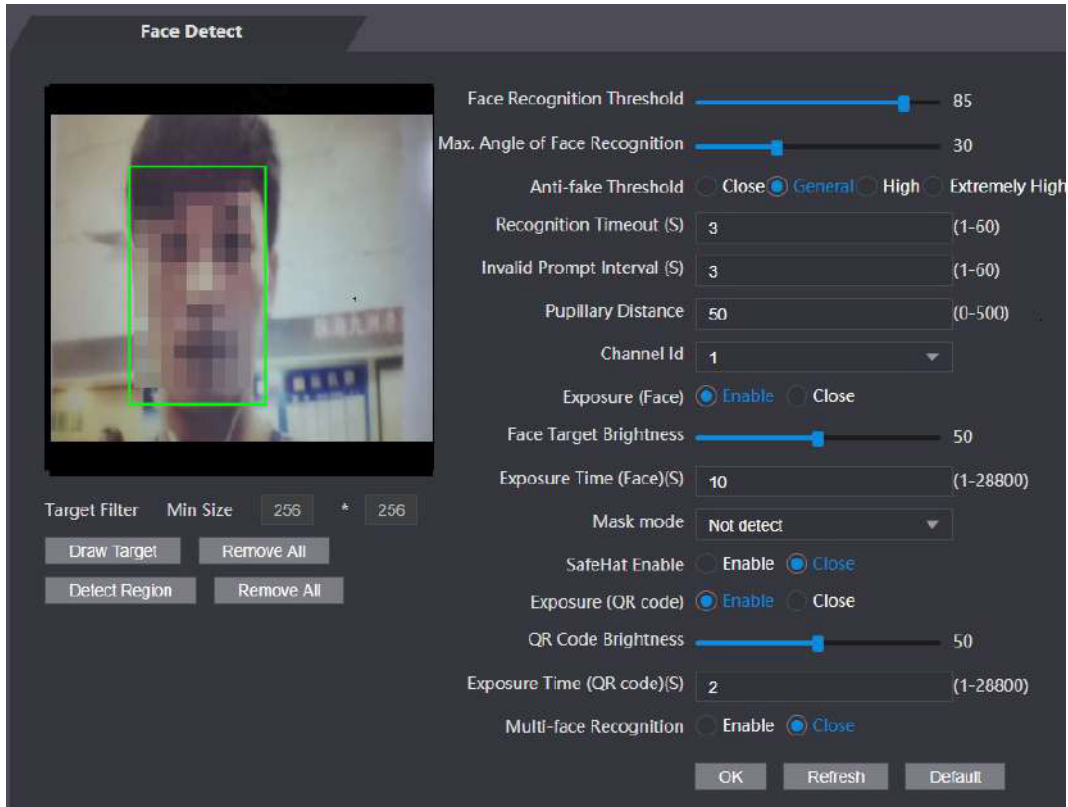
Figure 3-31 Face detect
