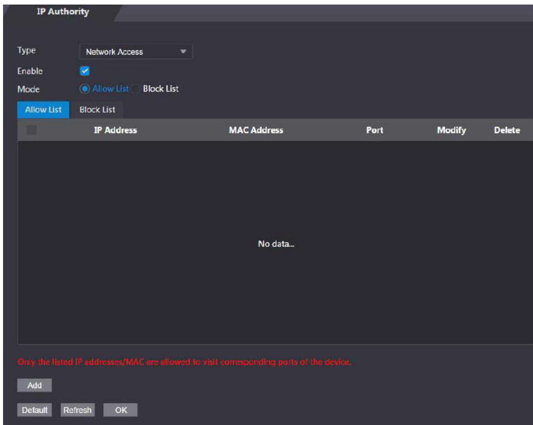
Figure 3-39 Network access
