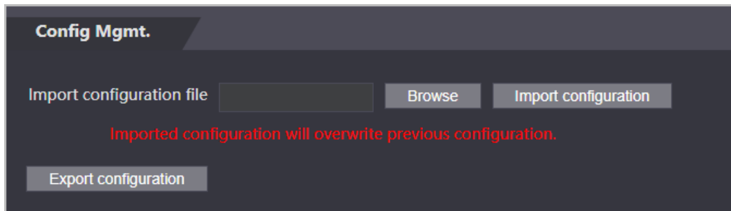
Figure 3-52 Configuration management
