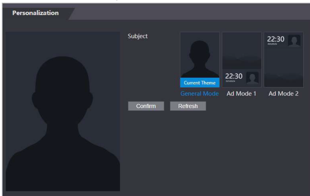
Figure 3-19 Theme
