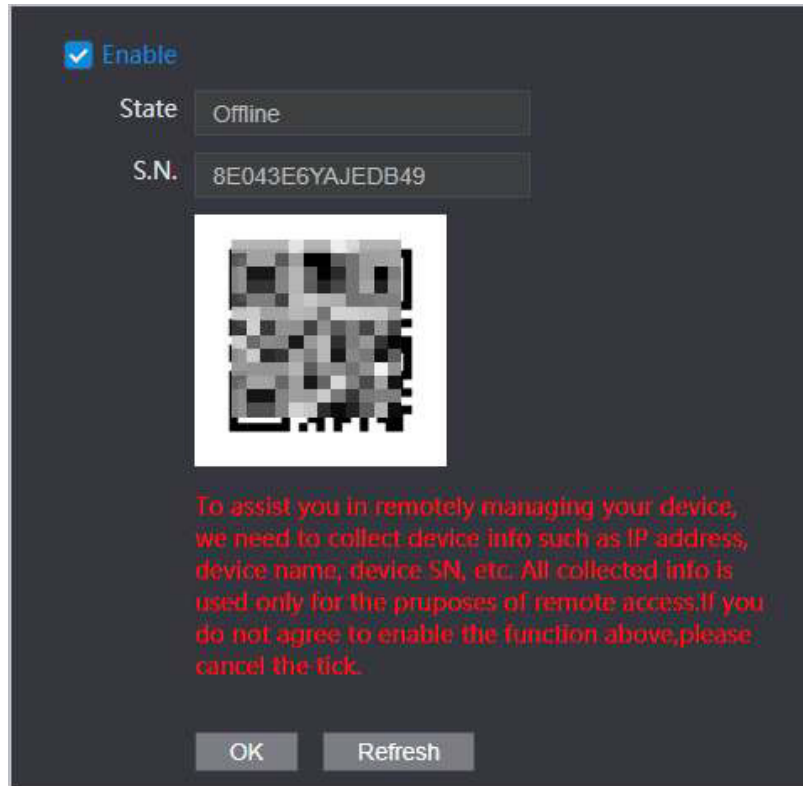
Figure 3-35 Cloud service
