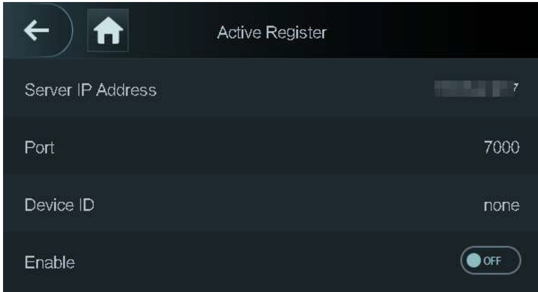
Figure 2-5 Auto register
