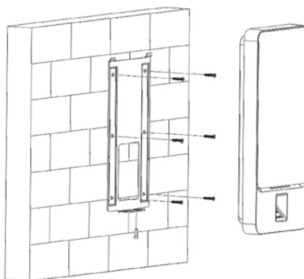
Figure 2-2 Installation diagram
