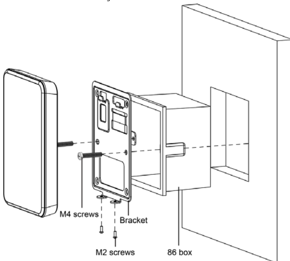
Figure 3-1 Wall mount
