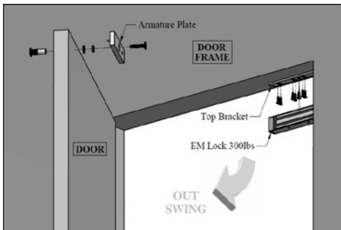
Explode View
